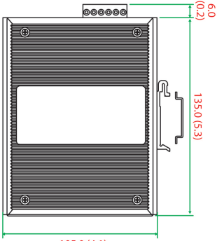
DIN-Rail Kit
