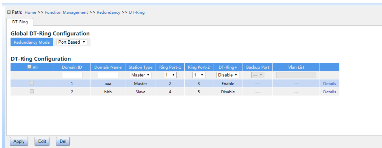
Figure 129 DT-Ring Configuration
