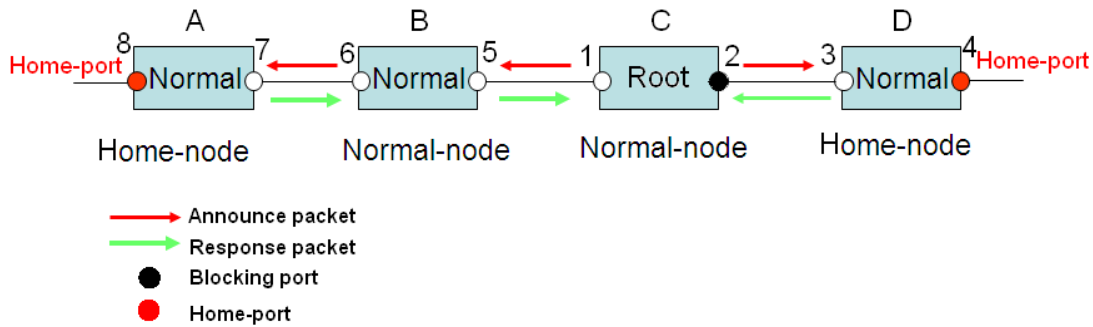
Figure 135 DHP Configuration
