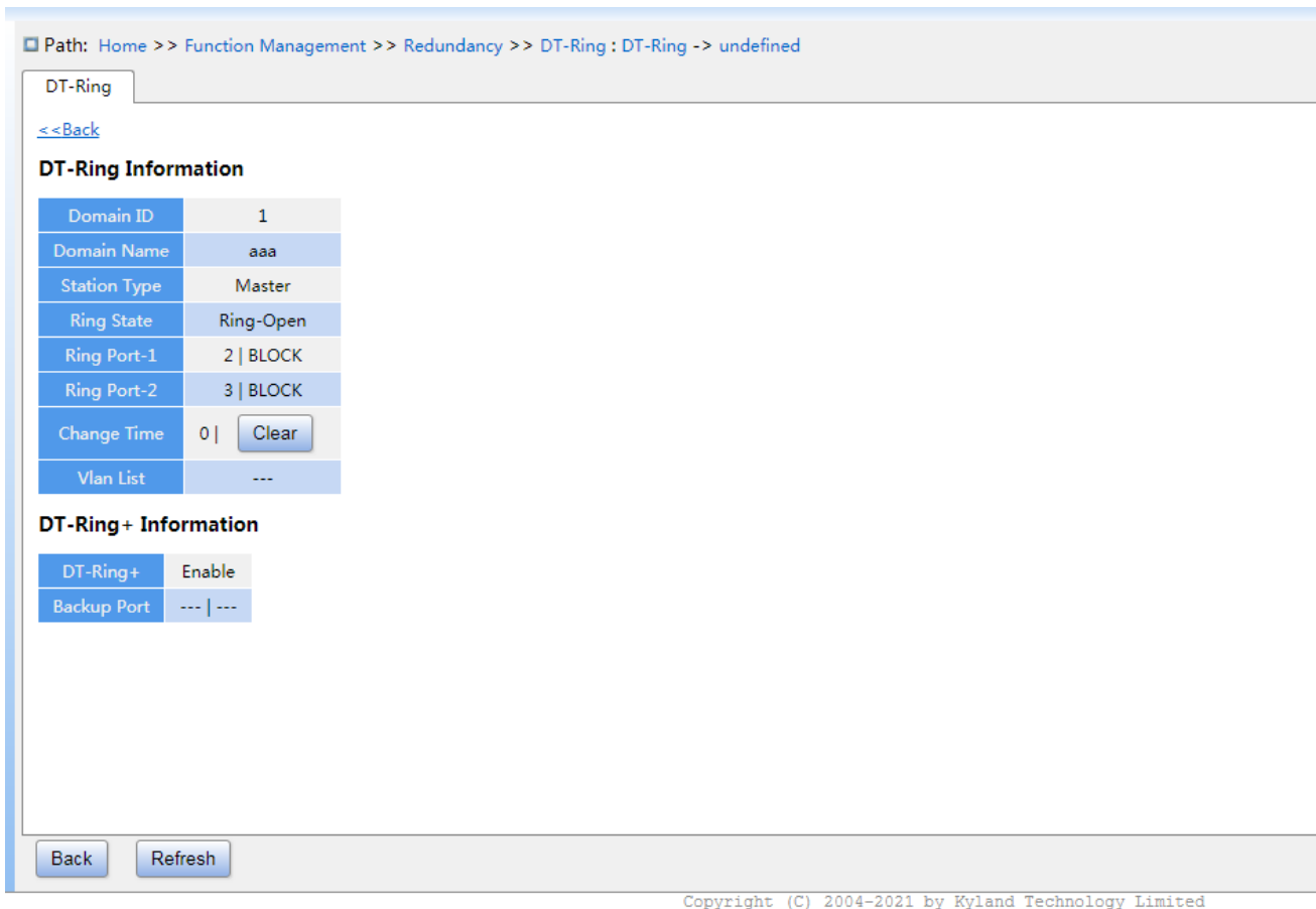
Figure 130 DT-Ring State
