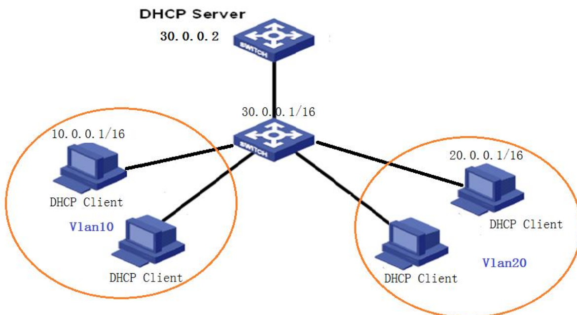
Figure 200 Client—Relay—Server Mode
