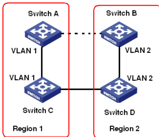
Figure 146 MSTP Topology
